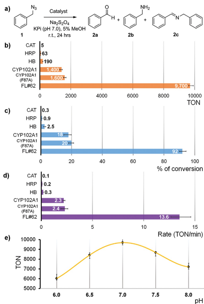
Figure 1. a) Catalytic activity of various hemoproteins in the oxidative deamination of benzyl azide (1) to benzaldehyde (2a). b, c) Reactions (400 \mu L) were conducted under anaerobic conditions with 10 mM BnN 3 , 10 mM Na 2 S 2 O 4 , and 1 \mu M protein for 24 h at room temperature. TON = nmol aldehyde/nmol catalyst. Product yield is based on conversion of 1 into 2a, as determined by GC. d) Reaction rates as determined over the first 10 min of the reaction. e) TON versus pH plot for FL#62 reaction.
